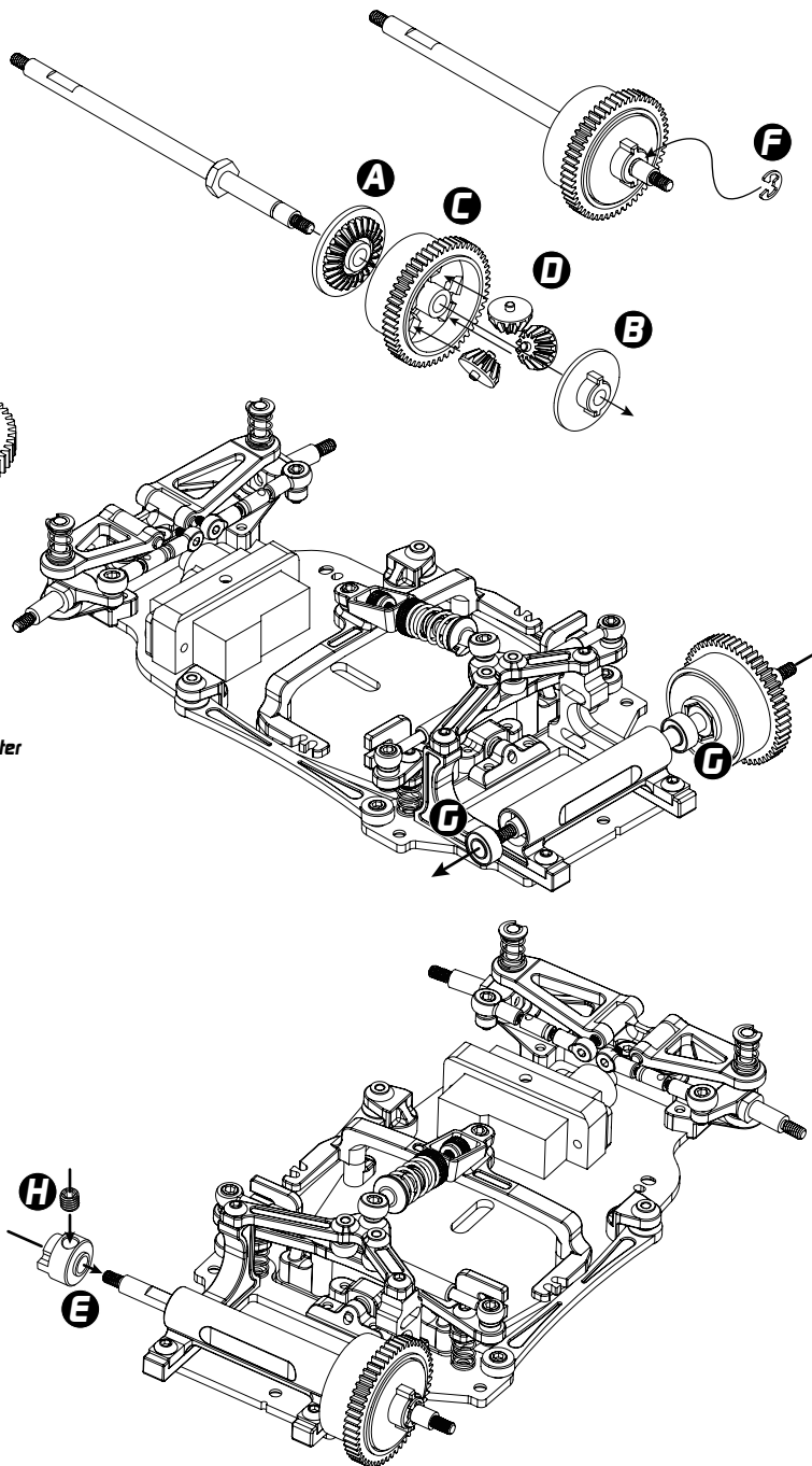
A XP-11275 - Composite Gear Diff
