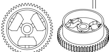
C XP-11275 - Composite Gear Diff
